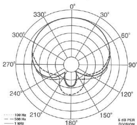
FIGURE 2 Polar Response
